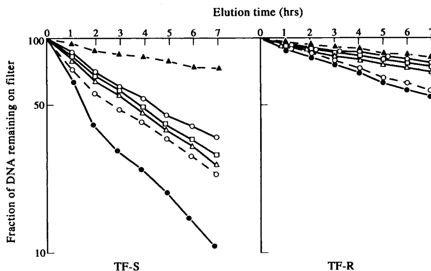
Fig. 4. Alkaline elution profiles of DNA single-strand breakage in TF-S and TF-R with BLM treatment. [ ^{14}\text{C} ]Thymidine-labelled cells were incubated with no drug ( \blacktriangle — \blacktriangle ) or 100 \mu\text{g}/\text{ml} of BLM at 37°C for 60 min ( \bullet — \bullet ). To permit DNA repair, cells were incubated at 37°C for 15 min ( \triangle — \triangle ), 30 min ( \square — \square ), and 60 min ( \circ — \circ ) or incubated at 4°C for 60 min ( \circ — \circ ) in BLM-free medium after BLM treatment. Then, cells were assayed for DNA strand breaks with the use of an alkaline elution technique described in Materials and Methods.
